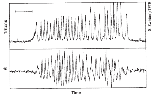
Escaping 1-MeV tritons (upper) resulting from magnetic perturbations \tilde{B} (lower) associated with magnetohydrodynamic modes. The energetic tritons are detected by particle detectors just outside the plasma boundary. An important issue is whether these perturbations or others, such as those associated with the \alpha -driven Alfvén mode, will eject a large fraction of the energetic \alpha -particles generated in TFTR deuterium-tritium plasmas. (Scale bar, 1 ms.)
